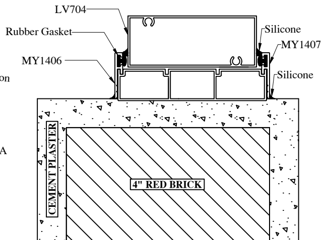
63.5MM & 76.2MM PROFILE SUBFRAME INSTALLATION SECTION VIEW
