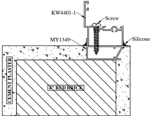
39MM PROFILE SUBFRAME INSTALLATION SECTION VIEW
