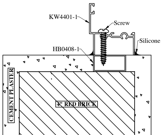
25.4MM PROFILE SUBFRAME INSTALLATION SECTION VIEW
